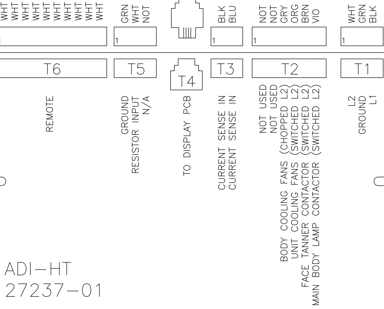
ELECTRONIC MAIN TIMER CONNECTOR DIAGRAM
